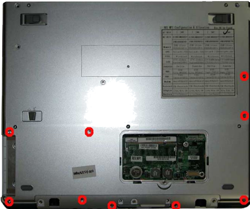
Fig. 24 Bottom Cover
